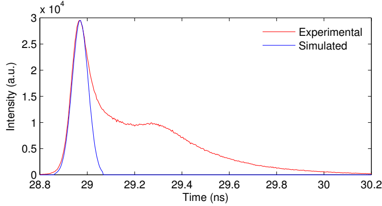
Figure 5.1: Simulated and practical laser pulse.
