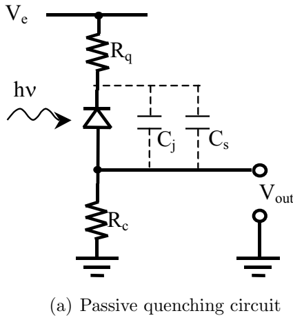
Figure 2.10: a) The simplest passive quenching circuit with quenching resistor R_q in the order of a few hundred k\Omega ; b) waveforms of the avalanche current (upper) and of the voltage applied to SPAD (lower).
