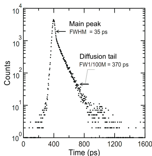
Figure 2.8: A typical time resolution curve of SPAD detector. The curve has a fast peak with FWHM=35 ps followed by a slow exponential tail with FWHM=80 ps. Adapted from [19].
