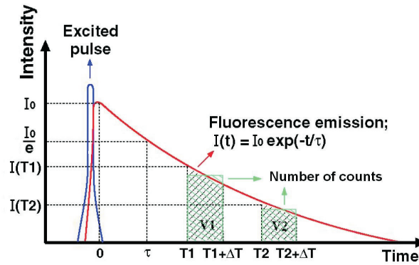
Figure 2.4: Mono-exponential fluorescence decay. Adapted from [11].
