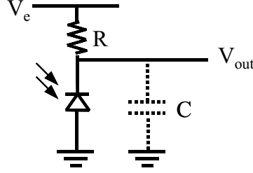
Figure 2.7: A simplified SPAD diagram.
