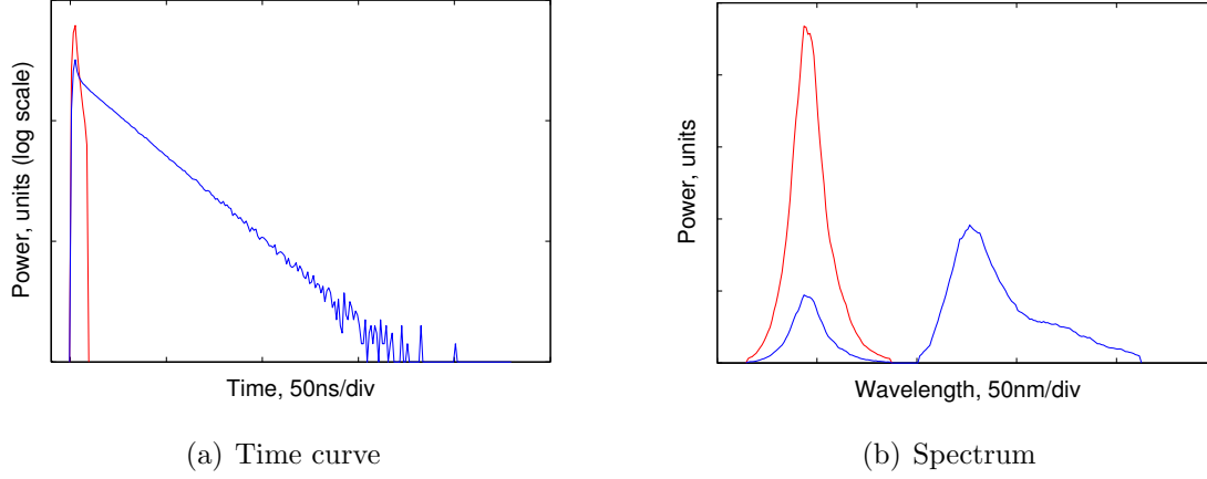
Figure 4.3: Fluorescence simulation. The time curve and the spectrum are shown for exciting (red curve) and fluorescent light (blue curve).
